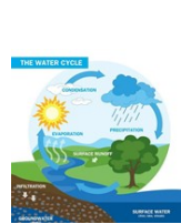
The water cycle
